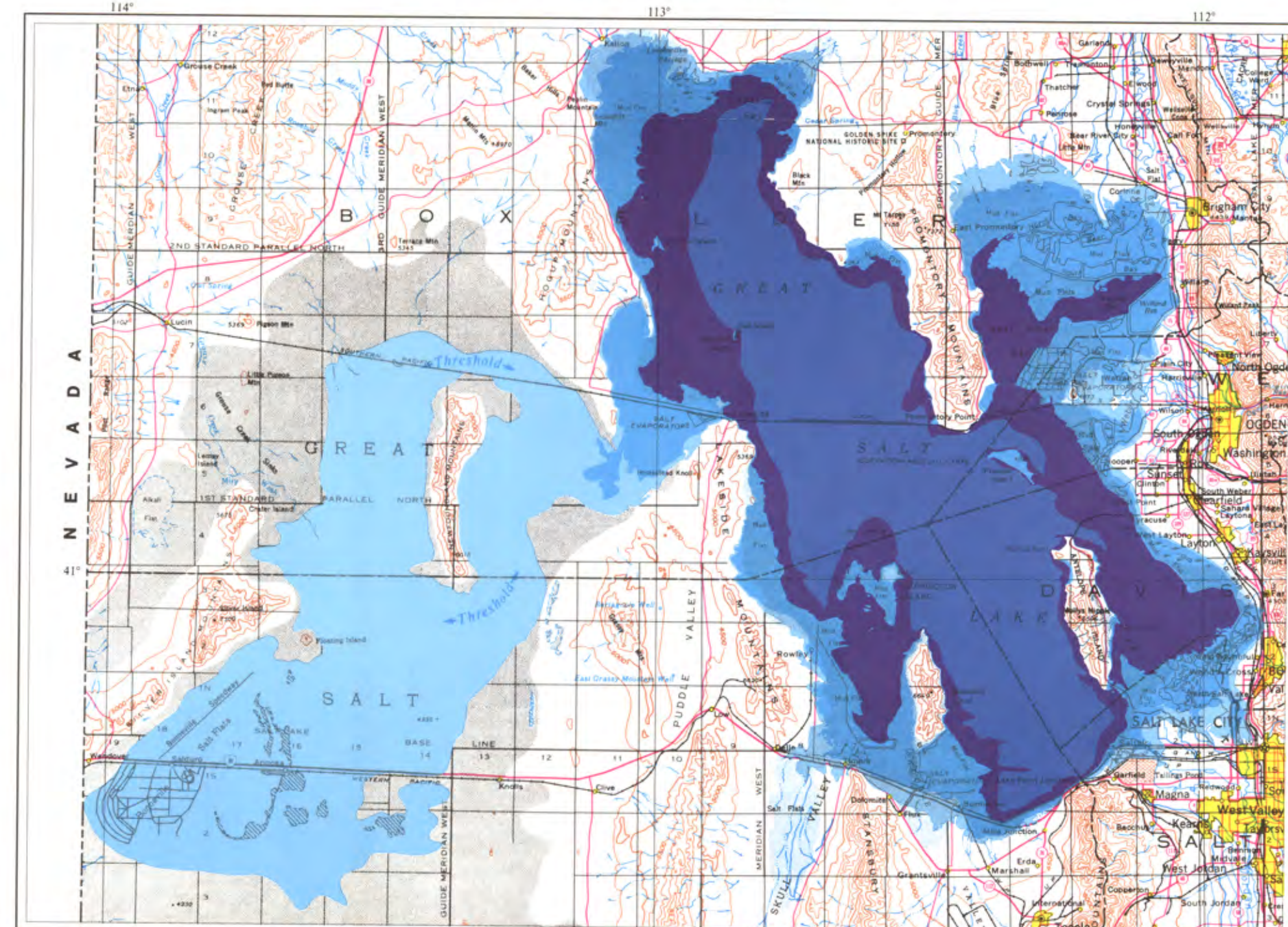
FIGURE 2. MAJOR LEVELS OF GREAT SALT LAKE. From highest to lowest, the levels depicted above are: Late Prehistoric High, approximately 4217 feet above sea level (a.s.l.) circa A.D. 1700(?); Historic High, 4212 feet a.s.l. in A.D. 1873; Historic Average, 4202 feet a.s.l.; and Historic Low, 4191 feet a.s.l. in 1963. See Table 1 for additional details.
